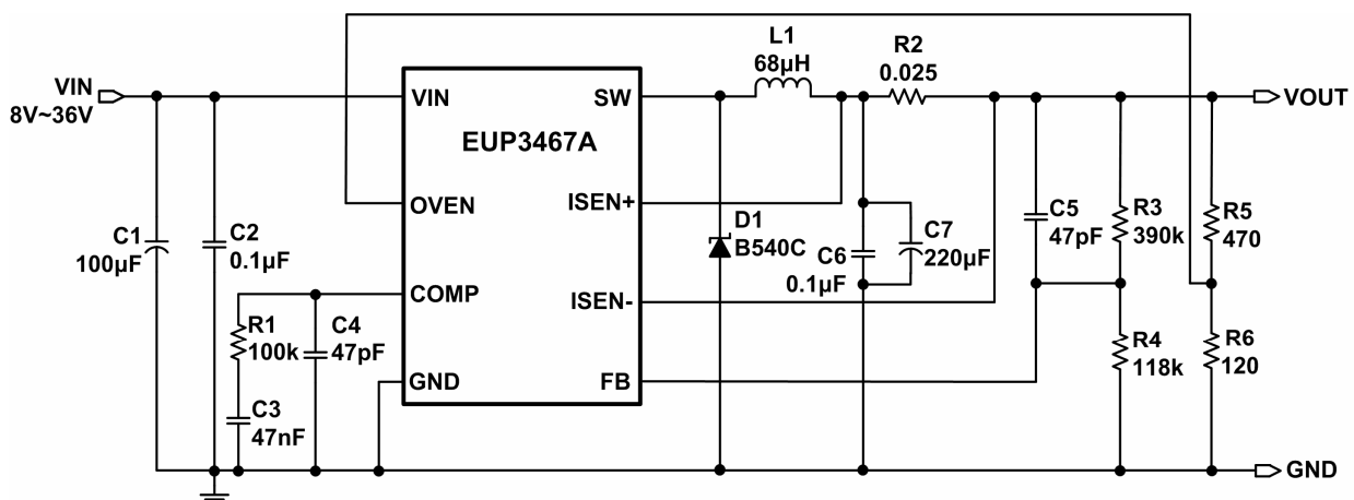
Figure 1. Application Circuit
