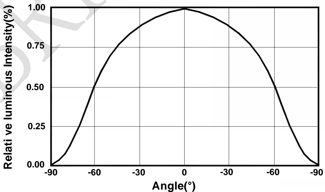
Typical Spatial Distribution
