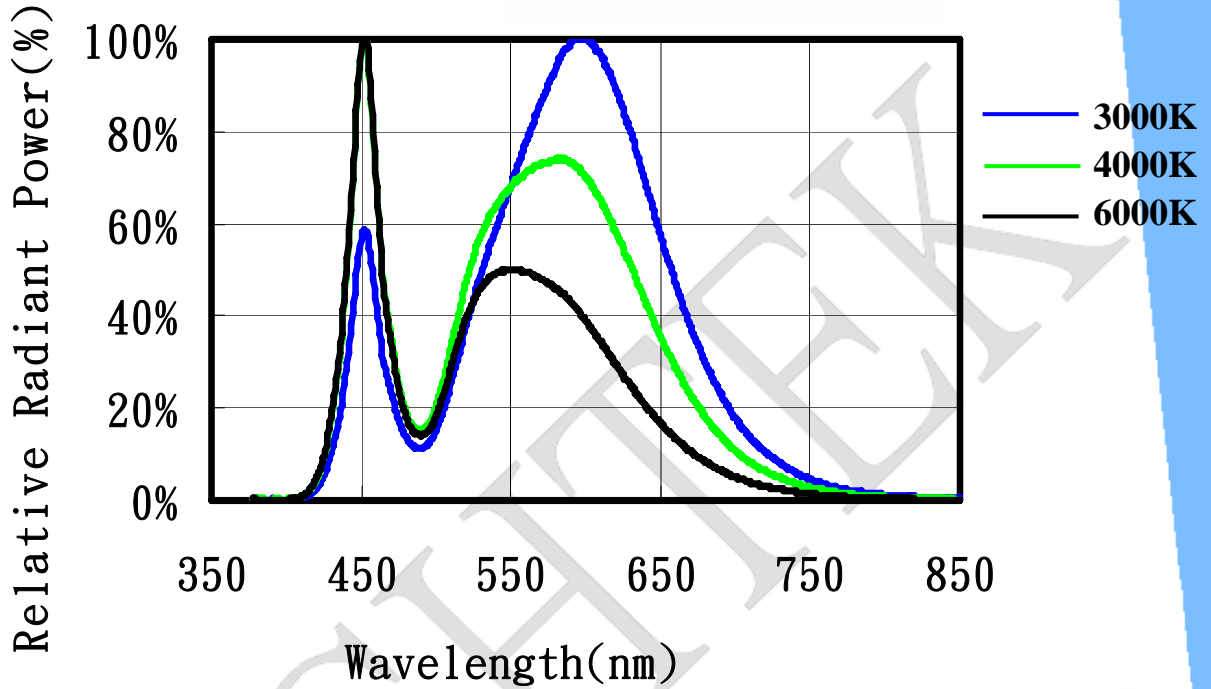
Relative Spectral Power Distribution
