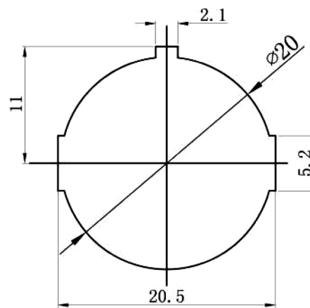
PANEL CUT-OUT
