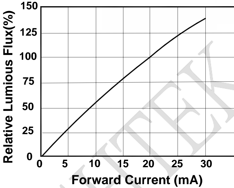
Relative Luminous Flux .Current
