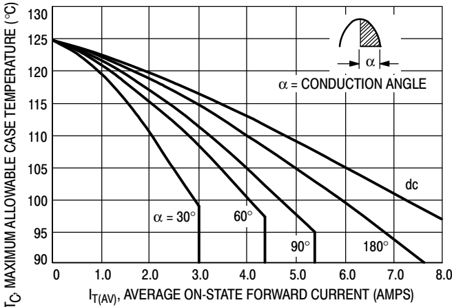
Figure 1. Current Derating
