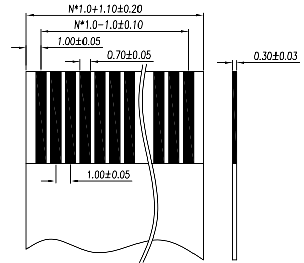
FPC Dimension Reference
