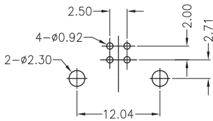
RECOMMENDED P.C.B HOLE LAYOUT TOP VIEW(TOLERANCE:±0.10)
